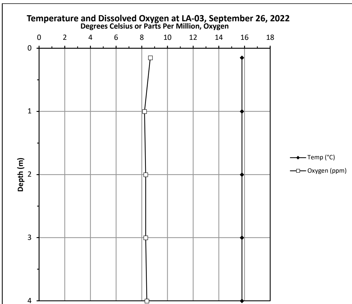
Figure 5 (cont.). Temperature and Dissolved Oxygen at Lake Almanor, Station LA-03, 2022
