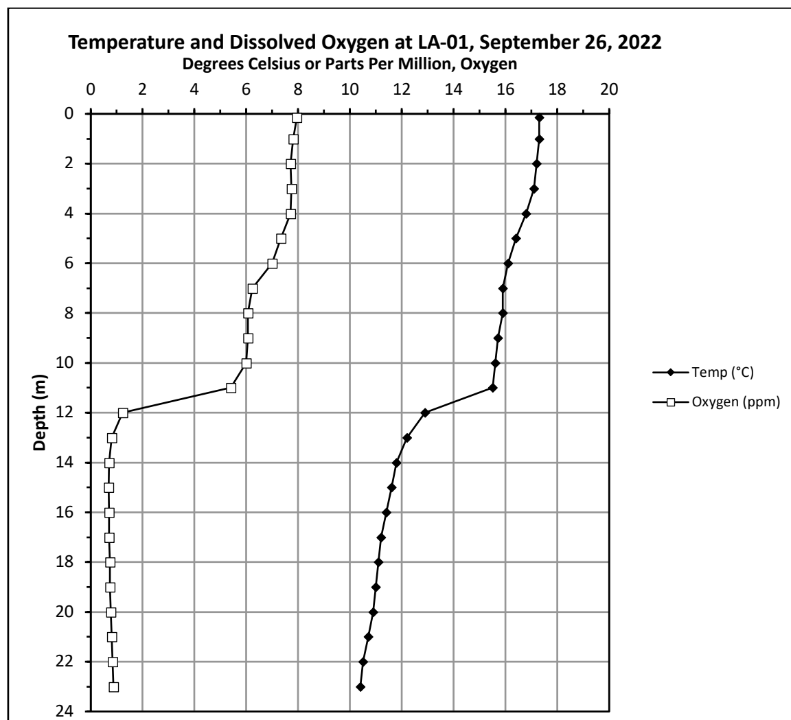
Figure 3 (cont.). Temperature and Dissolved Oxygen at Lake Almanor Station LA-01, 2022
