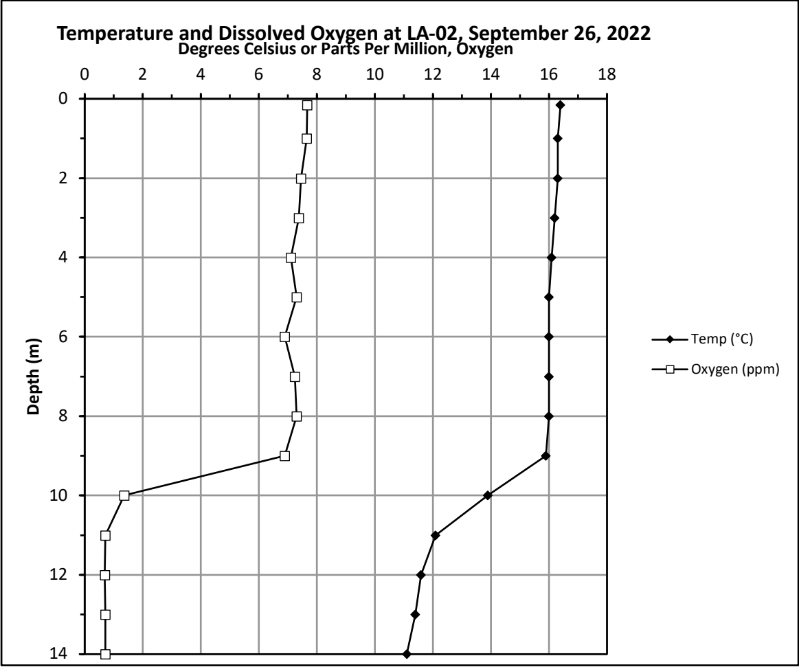
Figure 4 (cont.). Temperature and Dissolved Oxygen at Lake Almanor Station LA-02, 2022
